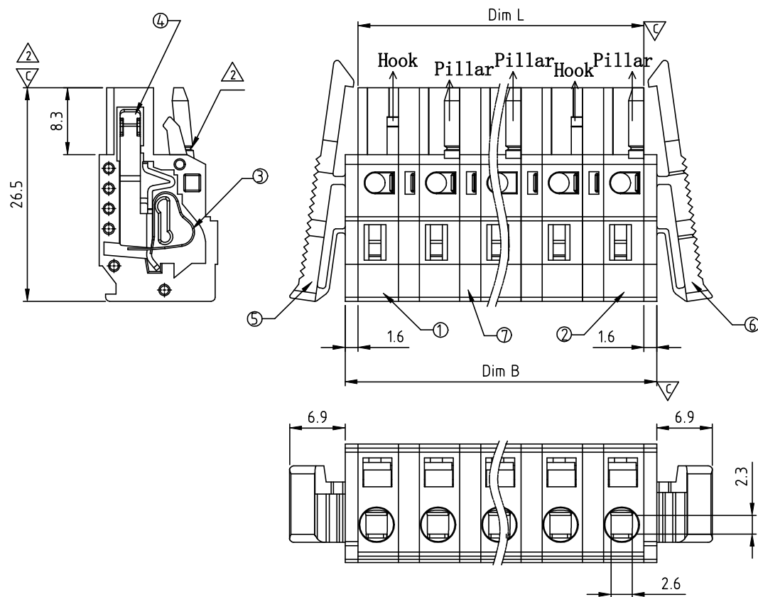
Layout of Hook and Pillar:
