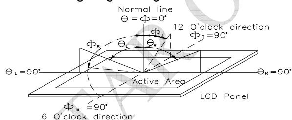
Fig 10.1. Definition of viewing angle
