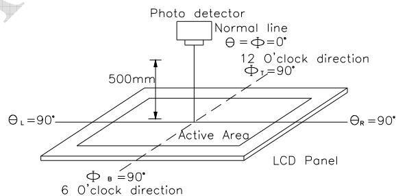
Fig 10.2. Optical measurement system setup
