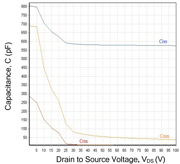
Capacitance Characteristics
