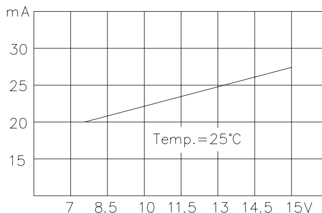
VOLTAGE-CURRENT CONSUMPTION
