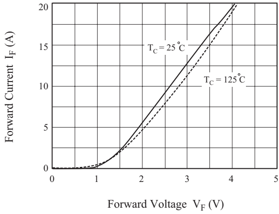
Fig 16. Forward Characteristics
