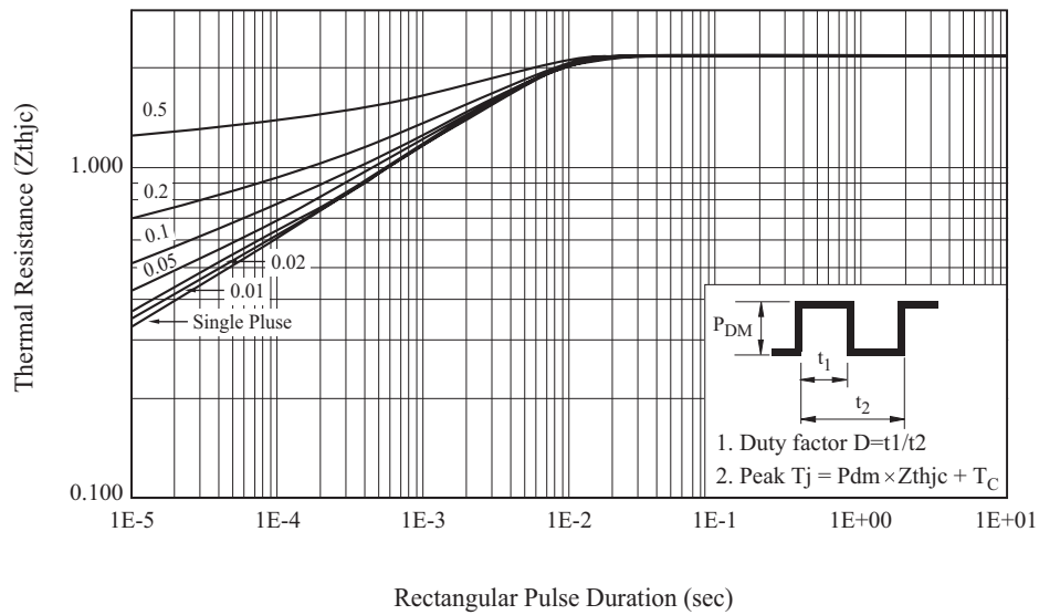
Fig 15. Transient Thermal Impedance of IGBT
