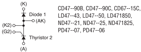
Diode 1, Thyristor 2 Modules
