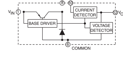
M57182N-315
