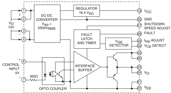
VLA502-01
