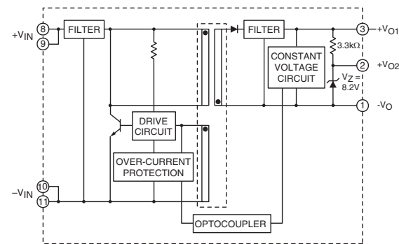
VLA106-15242, VLA106-24242
