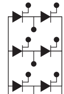
Three-Phase Full Controlled Bridge
