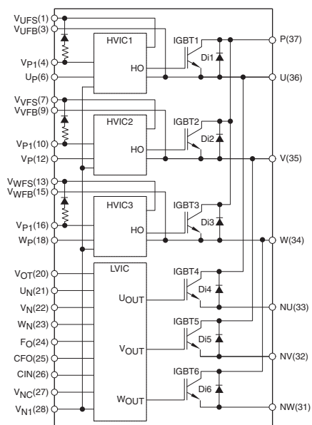
PSS20S71F6, PSS30S71F6, PSS50S71F6
