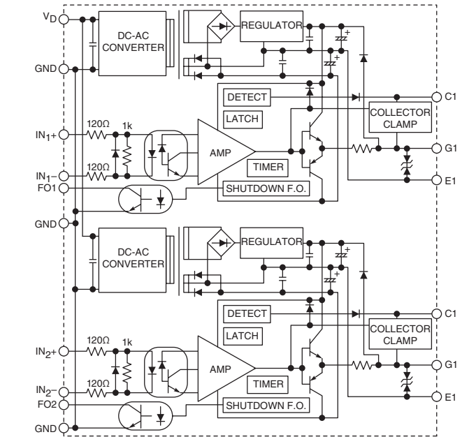
VLA553-01R, VLA553-02R
