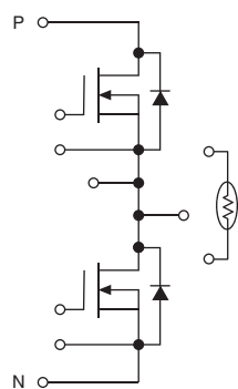
Dual MOSFET Module (By Paralleling)
