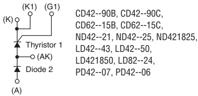
Thyristor 1, Diode 2 Modules
