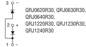
Dual Fast Recovery Diodes - Inverse Configuration
