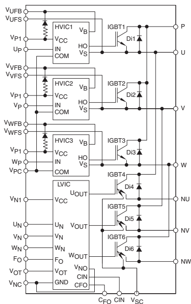
PSS05SA2FT, PSS10SA2FT, PSS15SA2FT, PSS25SA2FT, PSS35SA2FT, PSS50SA2FT
