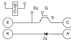
NX-Series Chopper IGBTs CM150EXS-24S, CM200EXS-24S, CM300EXS-24S
