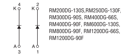
Dual High Isolation High Voltage Fast Recovery Diodes
