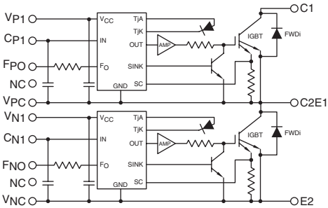
V1-Series, Duals PM400DV1A060, PM600DV1A060, PM800DV1B060, PM200DV1A120, PM300DV1A120, PM450DV1A120
