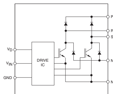
PS51787, PS51789
