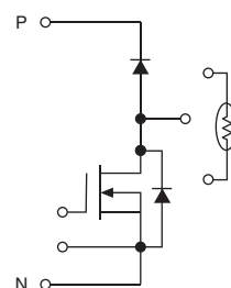
Chopper MOSFET Module (By Paralleling)
