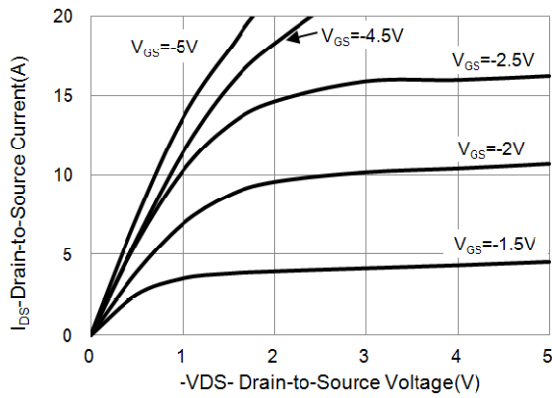
Fig.1 On-Region Characteristics
