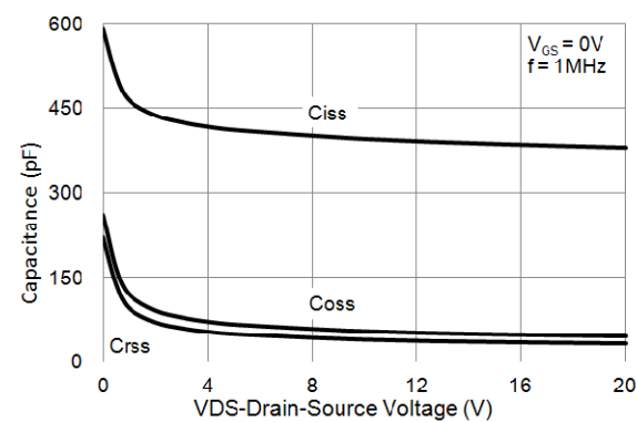
Fig.9 Capacitance vs. Drain-Source Voltage.
