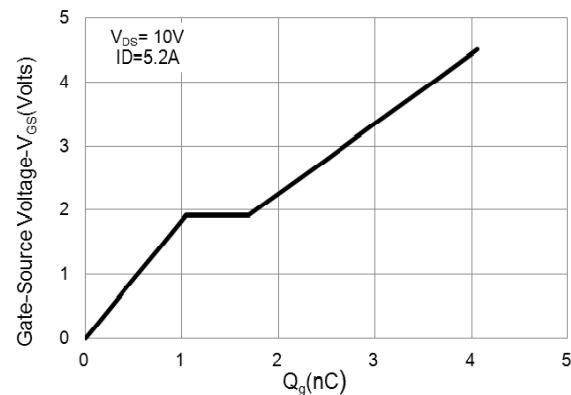
Fig.7 Gate-Charge Characteristics
