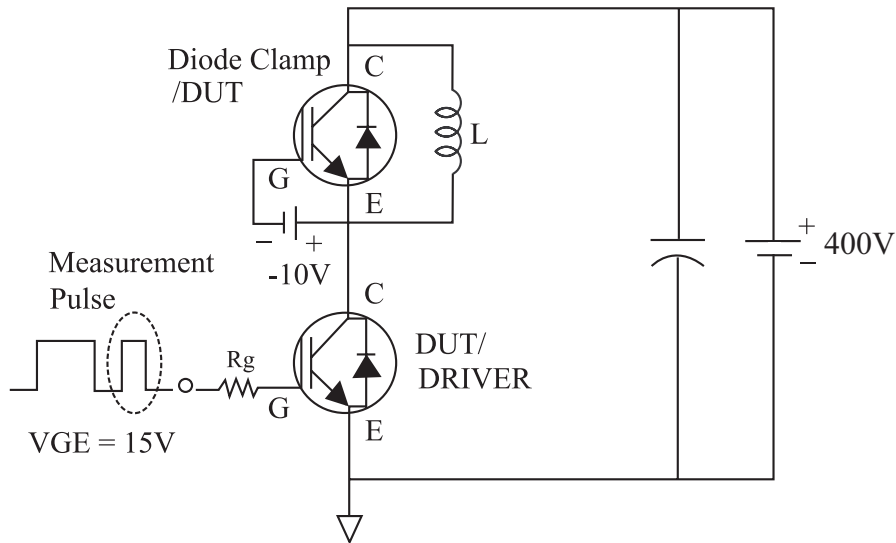
Fig 20. Definition Switching Time & Loss
