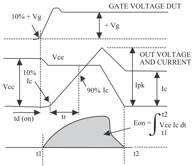
Fig 20. Definition Switching Time & Loss
