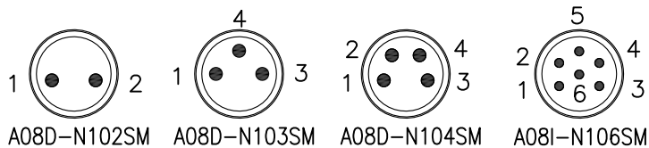
PIN ASSIGNMENT FRONT VIEW (前視圖)
