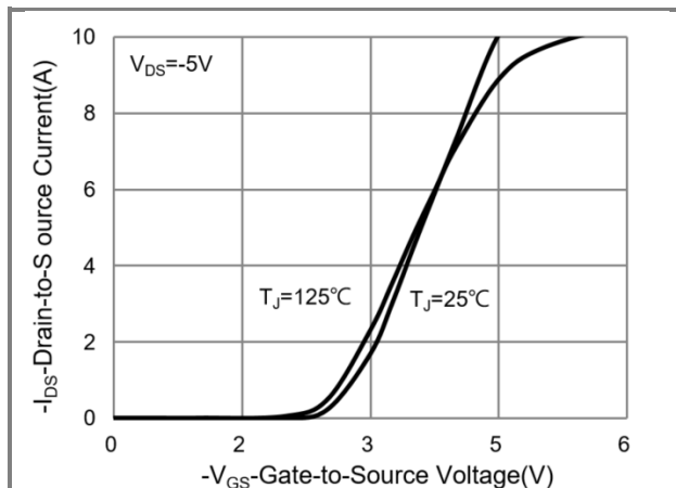
Fig.2 Transfer Characteristics
