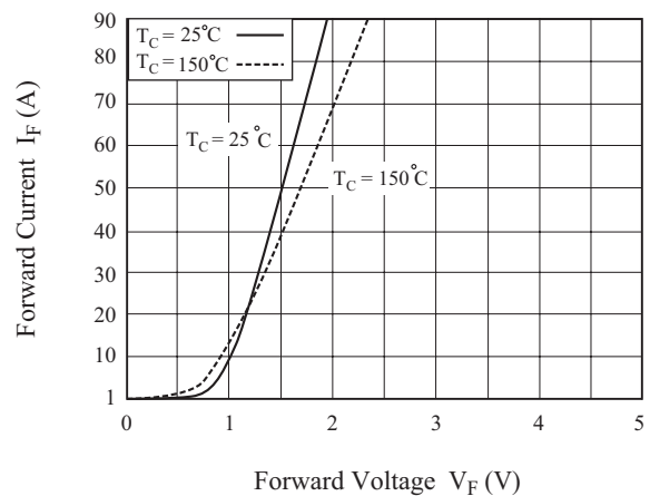
Fig 12. Forward Characteristics
