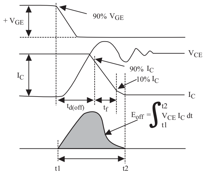
Fig 16. Definition Switching Time & Loss
