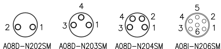
PIN ASSIGNMENT FRONT VIEW (前視圖)
