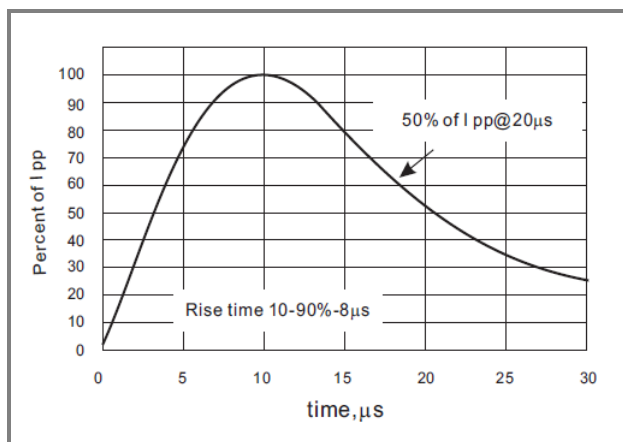
Fig.4 8/20 \mu s Pulse Waveform
