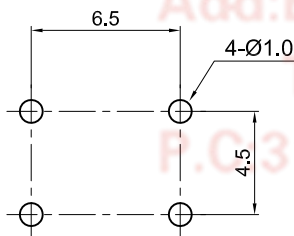
Recommend PCB layout Tolerance±0.05
