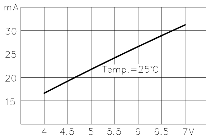
VOLTAGE-CURRENT CONSUMPTION
