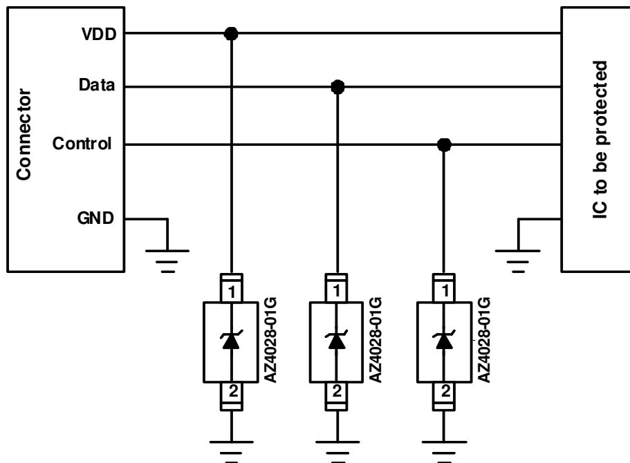
Fig. 1 ESD protection scheme by using AZ4028-01G.
