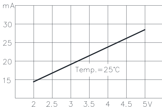
VOLTAGE-CURRENT CONSUMPTION
