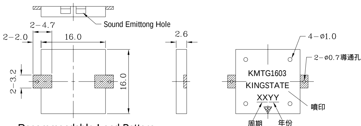
Recommendable Land Pattern
