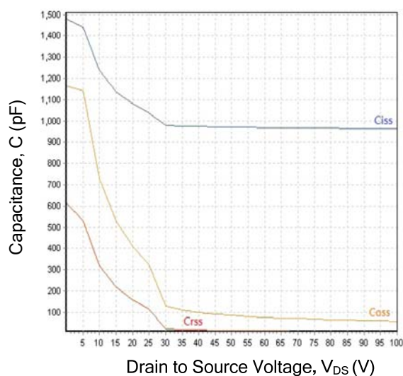
Capacitance Characteristics
