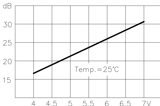
VOLTAGE-CURRENT CONSUMPTION
