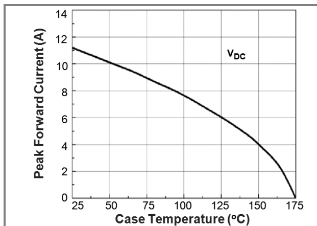
Fig.6 Current Derating
