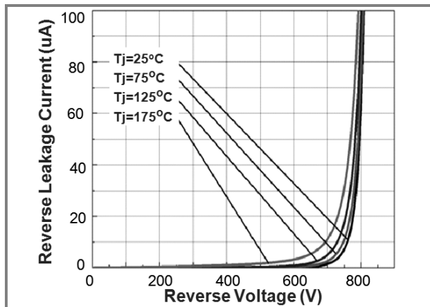
Fig.2 Reverse Characteristics
