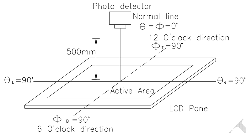
Fig. 12.2. Optical measurement system setup
