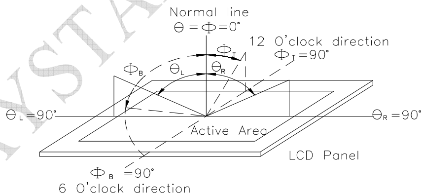
Fig. 12.1. Definition of viewing angle
